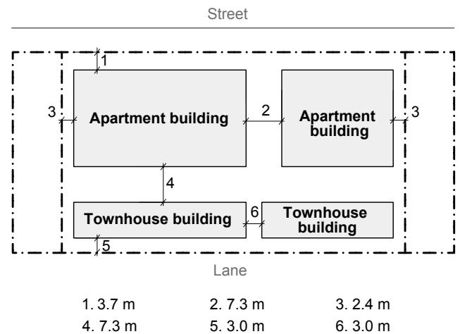
Diagram: Building placement – courtyard configuration
